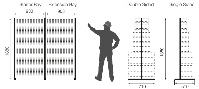
Louvre Rack dimensions (mm)
